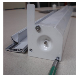
Place provided housing end cap on. secure with two screws.
